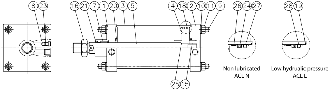
Standard (Lubricated type) (Ø125, Ø140, Ø150, Ø160)
