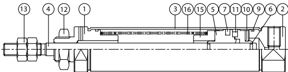
Single Acting Spring Return
